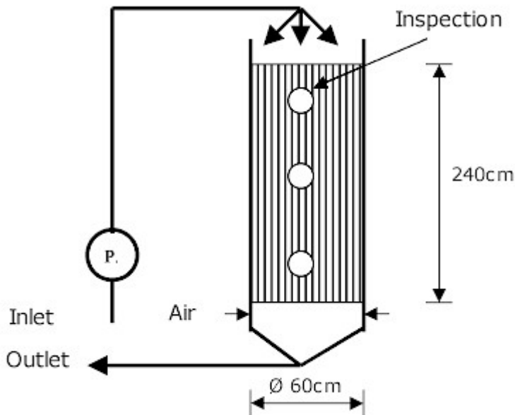
Figure 1: Test plant for trickling filter
