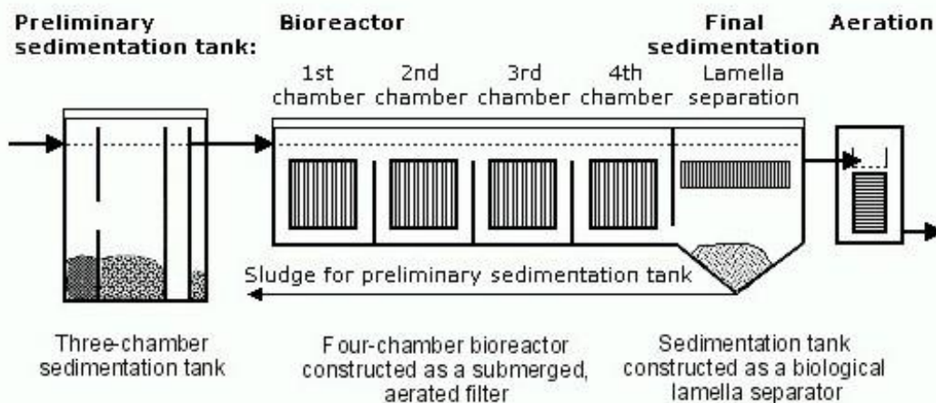
Cut of principle construction of submerged, aerated filter
