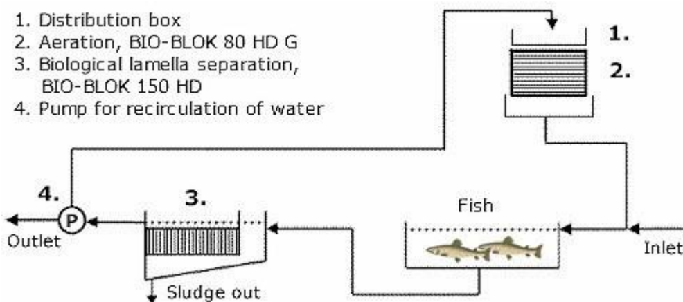
Recirculation plant
