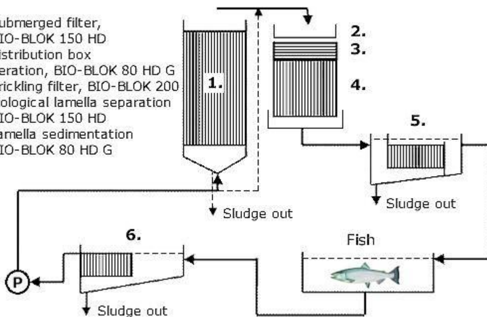
Recirculation Plant
